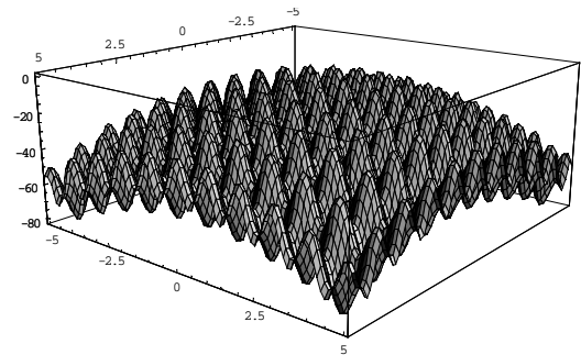
Fig.1 Rastrigin Function (Design Variable = 2)
