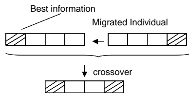
Fig.2 : Effects by migration
