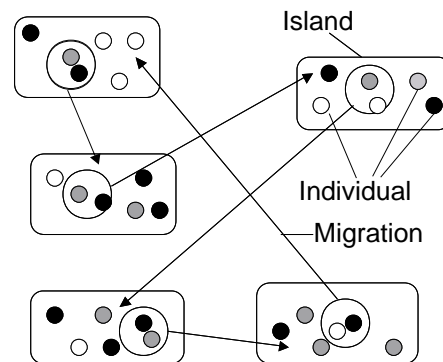
Fig.1 : Migration in DGA
