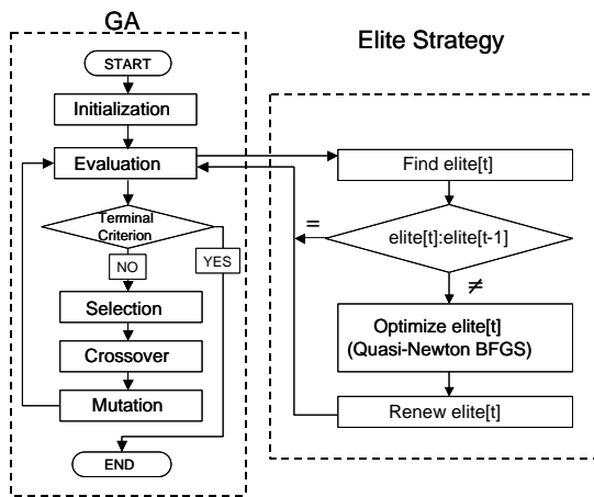
Fig.3 : Structure of proposed Hybrid GA
