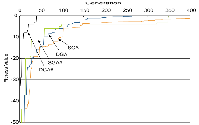
Fig.5 : Comparison of fitness value for Rastrigin Function with 4 approach
