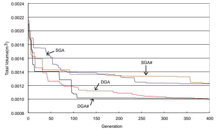
Fig.6 : Comparison of total volume for Truss Function with 4 approach
