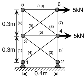
Fig.4 : The Setting of Truss Structure Optimization Problem(10-member truss structure)
