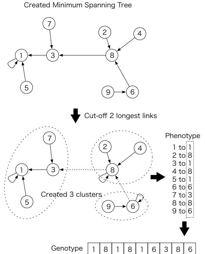
Figure 2: MST-based initialization
