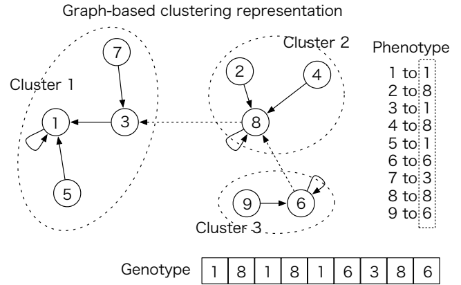
Figure 1: Graph-based representation
