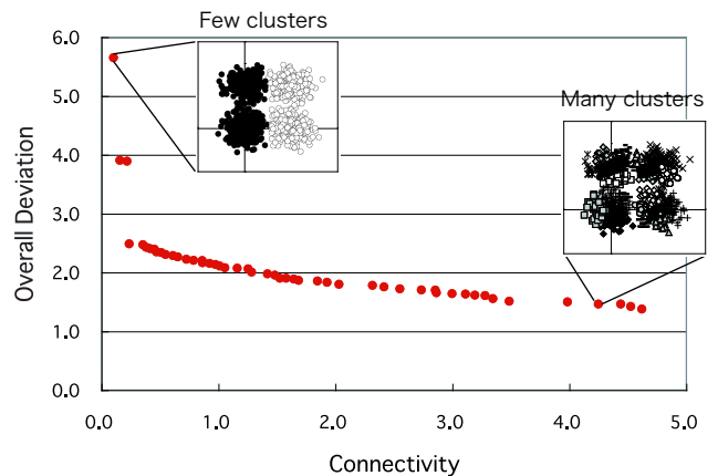
Figure 3: Pareto of MOCK
