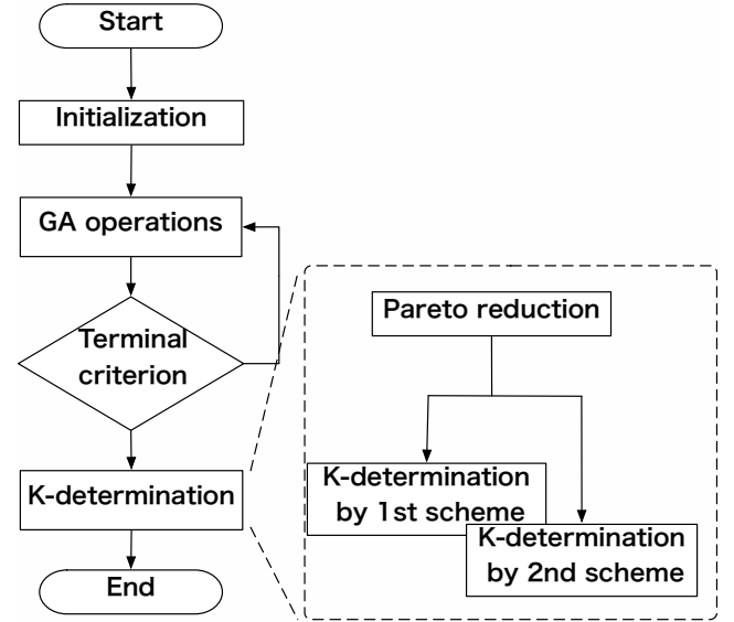
Figure 6: The flow of our automatic k-determination scheme
