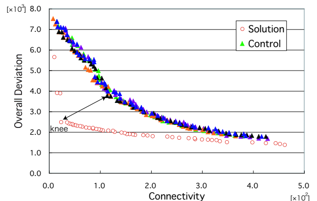
Figure 4: Automatic k-determination scheme of MOCK
