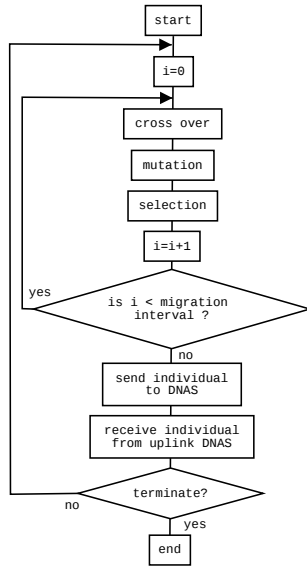
Figure 7. Flow chart for client side logic for the DGA model
