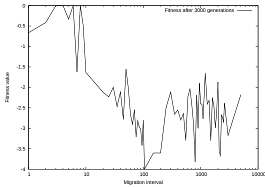
Figure 10. Fitness value after 3000 generations on 5-node set up, with 4 nodes representing islands of 100 populations each. Comparison is done based on different migration rates. Average of 5 tries.
