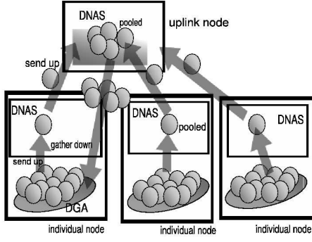
Figure 6. Implementation of DGA
