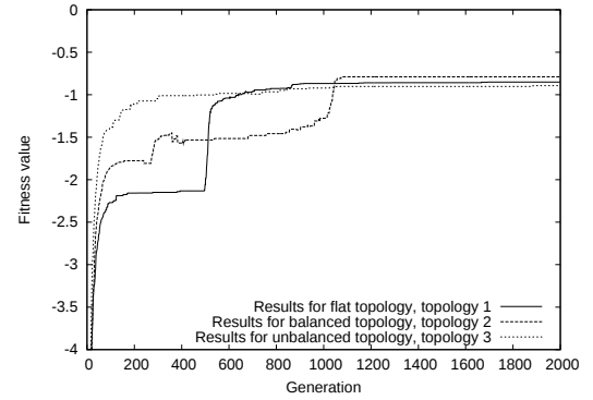
Figure 12. System having different static topologies, and running DGA process for 2000 generations
