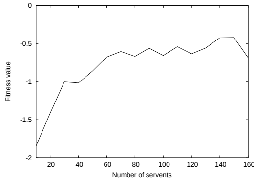
Figure 9. Fitness value after 2000 generation running with 10 to 160 nodes.
