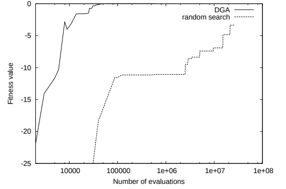
Figure 8. Searching progress of a random search program and a DGA program running on 10 nodes on a DNAS system
