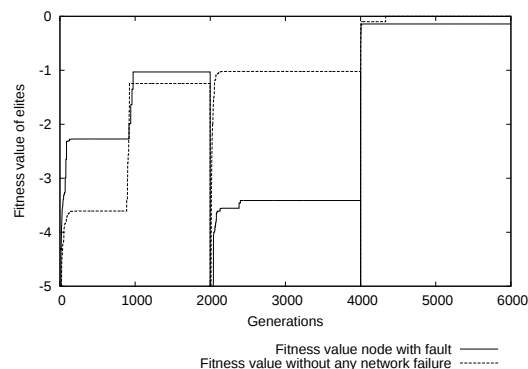
Figure 13. Comparison of DGA with resume at 2000 generations, running total of 6000 generations. Average value of fitness on all hosts. 7 hosts are used, with 6 islands. Comparing the effect of node with fault. One trial with manual fault in one host, and another without. Average of 10 tries.
