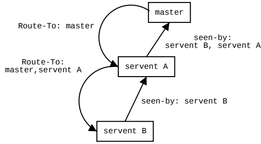
Figure 3. Information flow of Route-To: and Seen-By: message
